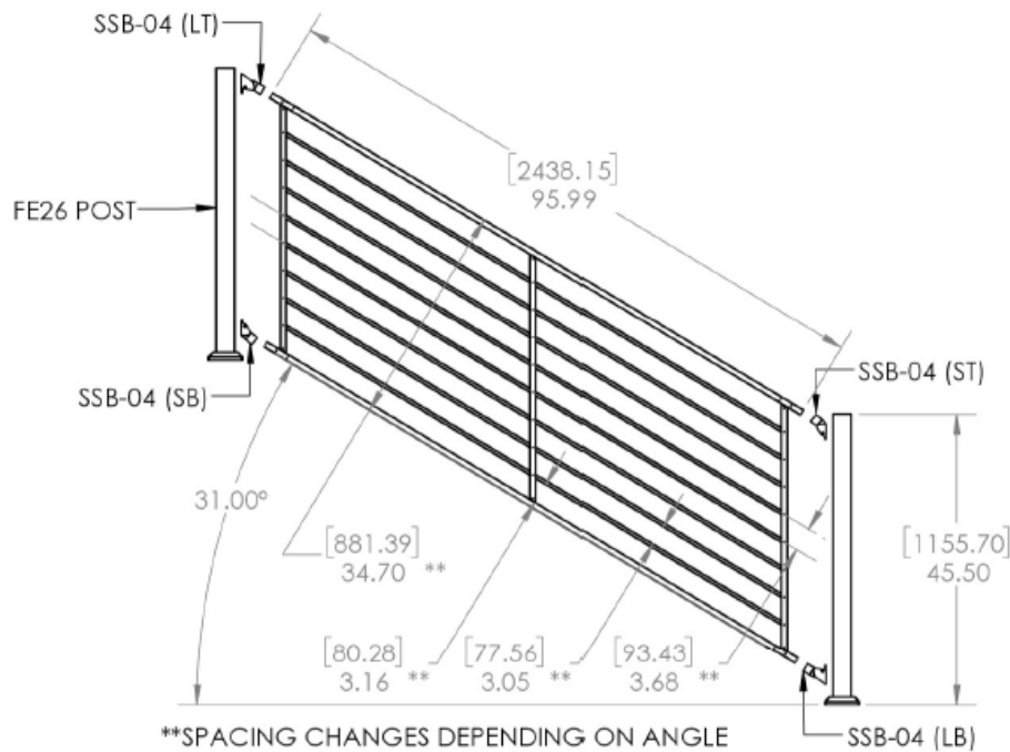
FIGURE 4 – FE 26 AXIS STAIR RAILING SYSTEM
