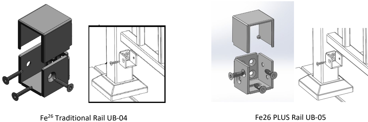
FIGURE 7 – UNIVERSAL BRACKETS AND INSTALLATION DETAIL
