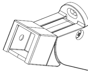
FIGURE 9 – SSB-04 SIMPLIFIED STAIR BRACKET FOR Fe 26 TRADITIONAL RAIL AND Fe 26 AXIS RAIL FOR ANGLES BETWEEN 29° AND 40°
