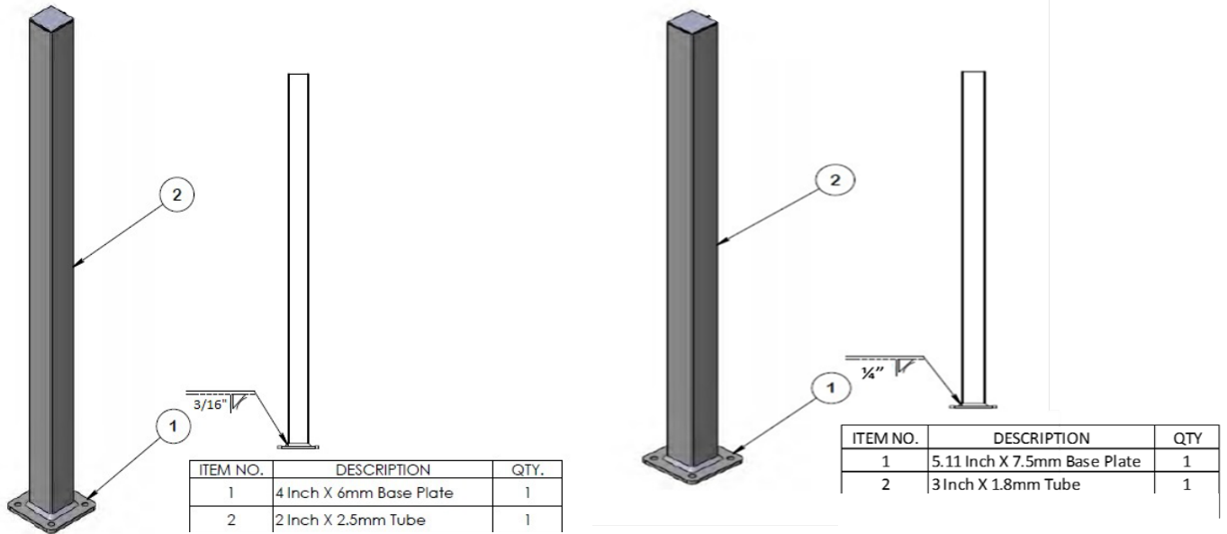
FIGURE 11 – STEEL POST MOUNTS AND BASES
