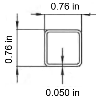
Fe 26 PLUS Railing Baluster
