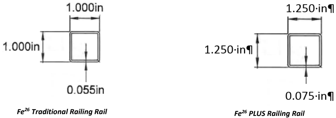
FIGURE 5 – RAILING PROFILES
