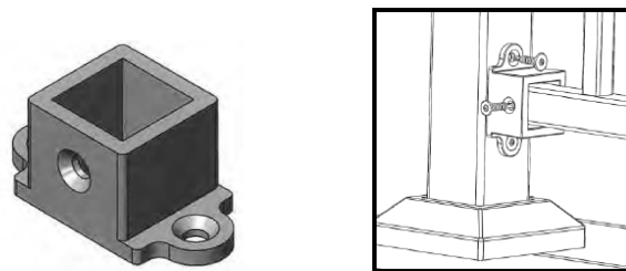
FIGURE 6 – CB-04 COLLAR BRACKET AND INSTALLATION DETAIL FOR THE Fe 26 TRADITIONAL RAIL
