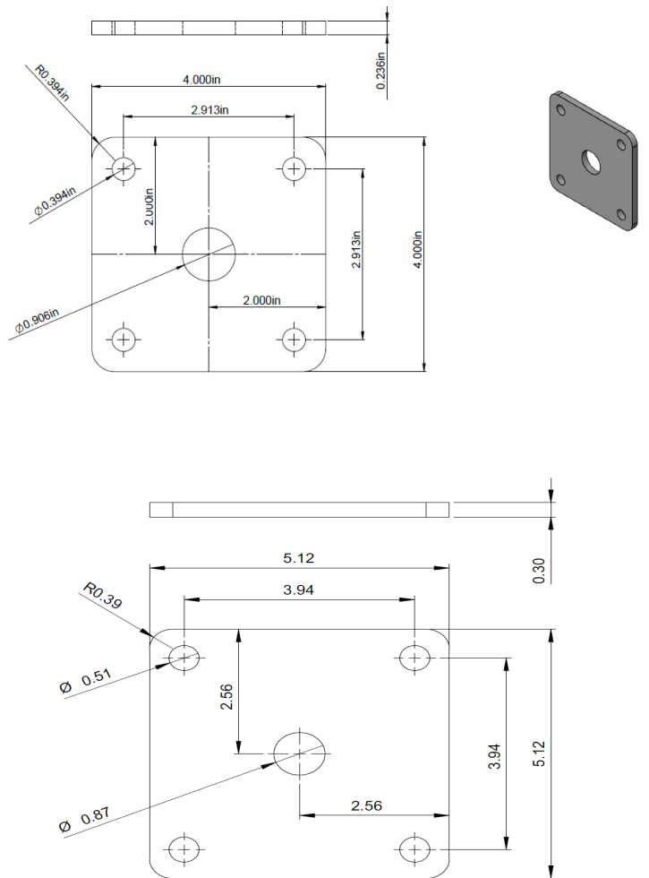
FIGURE 12 – FE 26 2" AND 3" POST BASE PLATES
