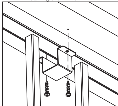
Top cap installation when installing a drink rail
