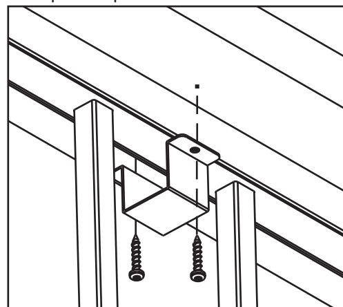
Top cap installation when using cap rail clips to install a drink rail
