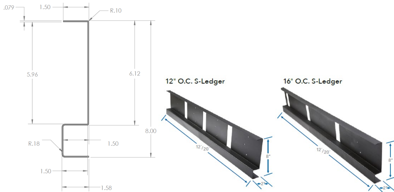
FIGURE 3 – LEDGERS
