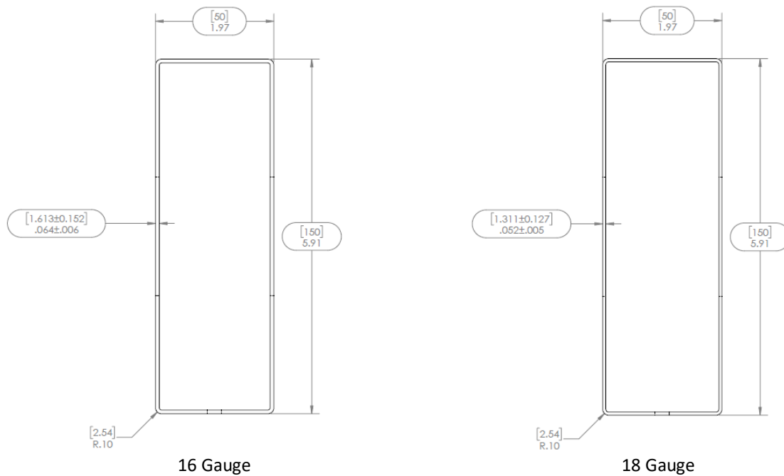
FIGURE 2 – STEEL JOISTS
