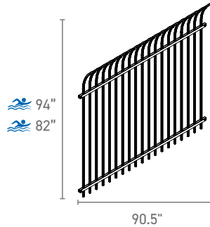
Two Rail Panels
